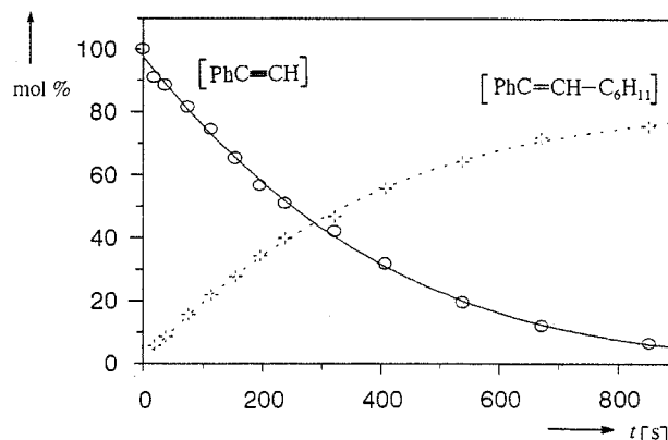
Figure 1. Conversion of phenylethyne (1) and formation of the addition products 4 [(Z)-4, (E)-4] at 340°C and 200 bar (5.82 M cyclohexane)
