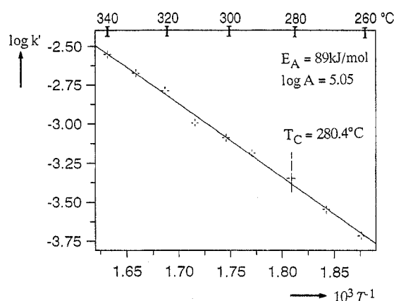
Figure 3. Temperature dependence of the pseudo-first-order rate constant of the addition of cyclohexane to phenylethyne ( 1 ) (Arrhenius plot)
