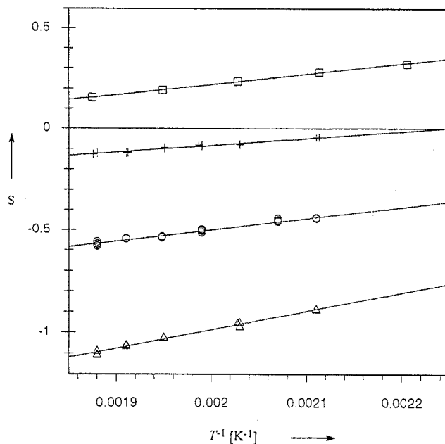
Figure 2. Temperature dependence of the stereoselectivity S of the hydrogen transfer from cyclohexane to cyclic radicals 2a–d ( S = \lg([(Z)-\mathbf{3}]:[(E)-\mathbf{3}]) ). □ = Me, + = Et, ○ = c -C 6 H 11 , Δ = t Bu
