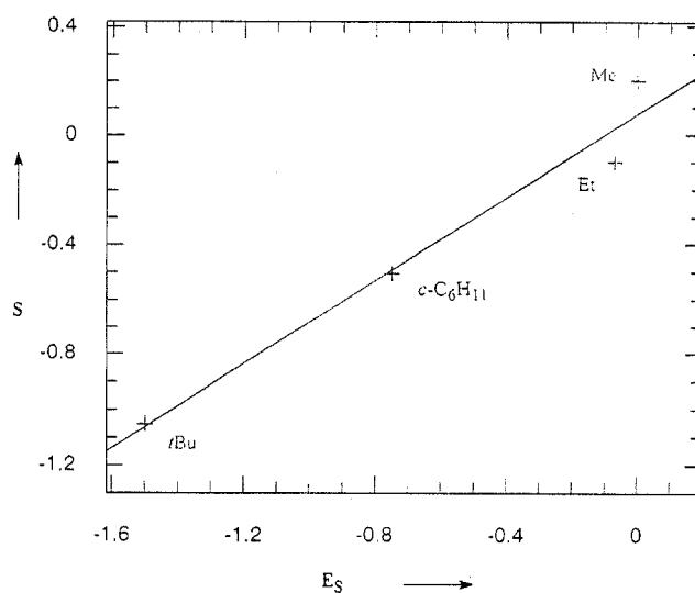
Figure 3. Correlation of the stereoselectivity S of the hydrogen transfer from cyclohexane to radicals 2a–d (200°C) with steric substituent constants E_s of the alkyl substituents ( S = \lg([(Z)-\mathbf{3}]:[(E)-\mathbf{3}]) )
