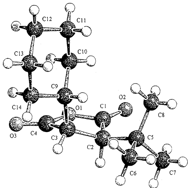
Figure 1. Schakal plot of (Z)- 3d . Selected bond lengths [pm] and inter-bond angles [°]: C(1)–C(2) 149.6(5), C(2)–C(3) 154.4(5), C(3)–C(4) 150.5(5), C(1)–O(1) 138.7(5), C(4)–O(1) 139.3(6), C(2)–C(5) 154.1(4), C(5)–C(6) 152.3(5), C(5)–C(7) 153.4(5), C(5)–C(8) 152.7(4), C(3)–C(9) 154.8(4), C(11)–C(12) 149.3(6); C(1)–C(2)–C(3) 102.9(3), C(2)–C(3)–C(4) 100.7(3), C(1)–C(2)–C(5) 118.0(3), C(3)–C(2)–C(5) 123.6(2), C(2)–C(3)–C(9) 118.6(2), C(4)–C(3)–C(9) 109.6(3)
