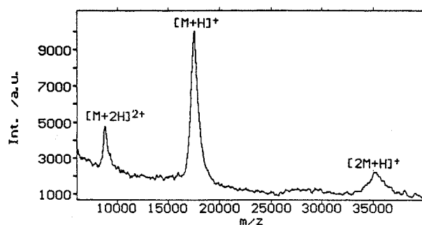
Fig. 2. MALD mass spectrum of myoglobin (horse skeletal muscle) using 3-aminoquinoline as matrix. The spectrum is accumulated from 30 single shots
