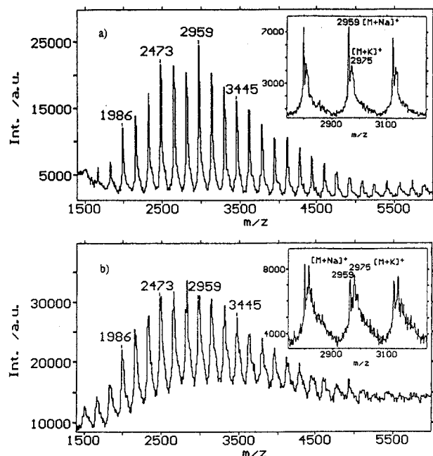
Fig. 1. Matrix-assisted laser desorption mass spectrum of chicory inulin using a) 3-aminoquinoline and b) 2,5-dihydroxybenzoic acid as matrix. The spectra are accumulated from a) 27 and b) 50 single shots. Intensity in arbitrary units, molecular weight M , in Da ( m/z )
